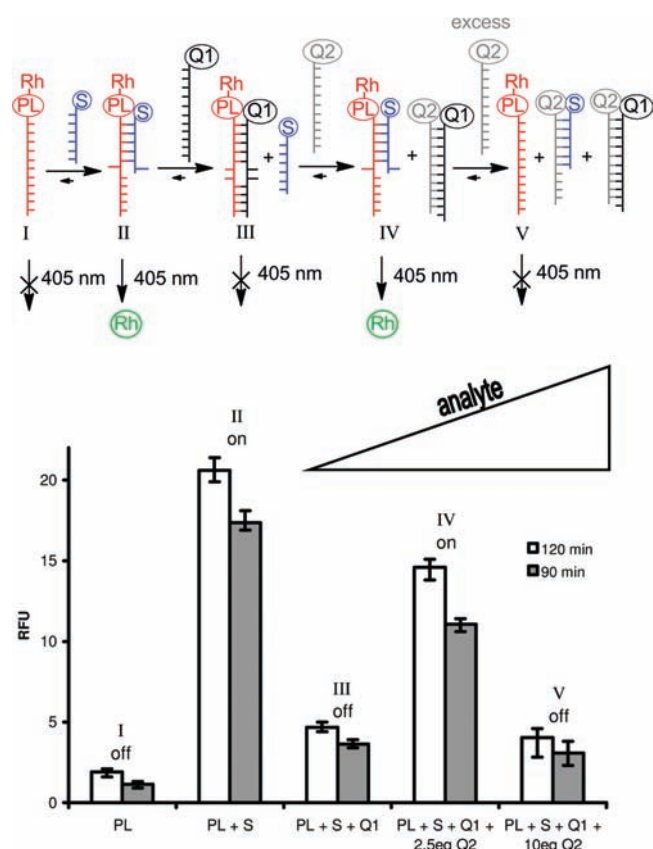
Figure 4. Fluorescence measurements of photoreaction after 90 and 120 min with different amounts (0–2.5 \mu\text{M} ) of 10-mer Q2 (Lys(Q)-TG*AC*TA*CA*AC*-Arg) under irradiation with an LED (405 nm, 100 mW) using 250 nM PL [Lys(PL)-TG*AC*TC*GA*AC*T-Arg], 250 nM S (Arg-TAG*TCA*-S), 375 nM Q1 (Arg-AG*TTG*TAG*TCA*-Q), and 625 nM (2.5 equiv) or 2500 nM (10 equiv) Q2 (Lys(Q)-TG*AC*TA*CA*AC*-Arg). Buffer: 10 mM PBS (pH 7.4), 154 mM NaCl, 25 mM MgCl 2 , 0.05% Tween. Data points are averages of three experiments, and error bars represent standard deviations.
